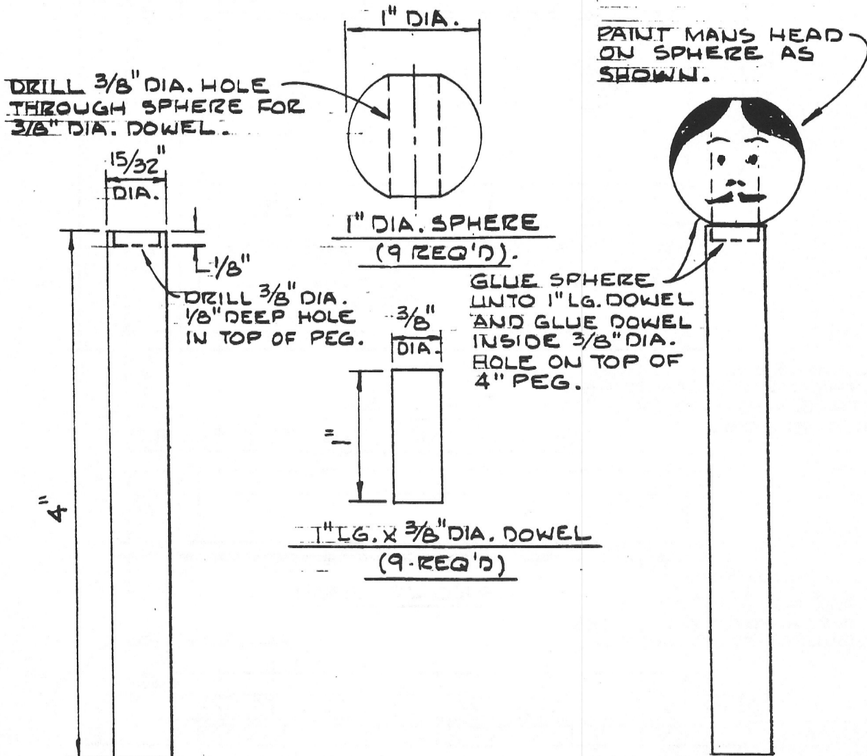
ASSEMBLY OF SPHERE TO 4" PEG (9 REQ'D)
