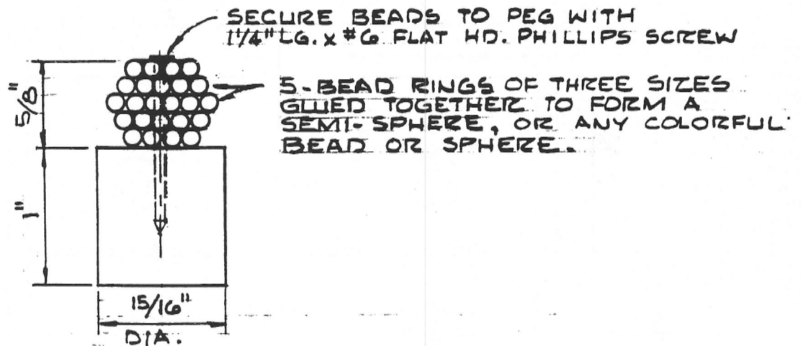
1" X 1 1/16" DIA. PEG DETAIL (9 REQ'D).
