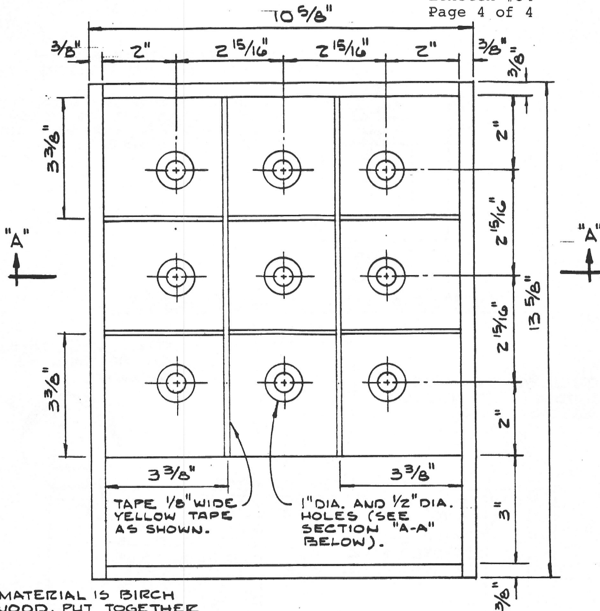
TOP VIEW OF TIC-TAC-TOE TOY BOARD
